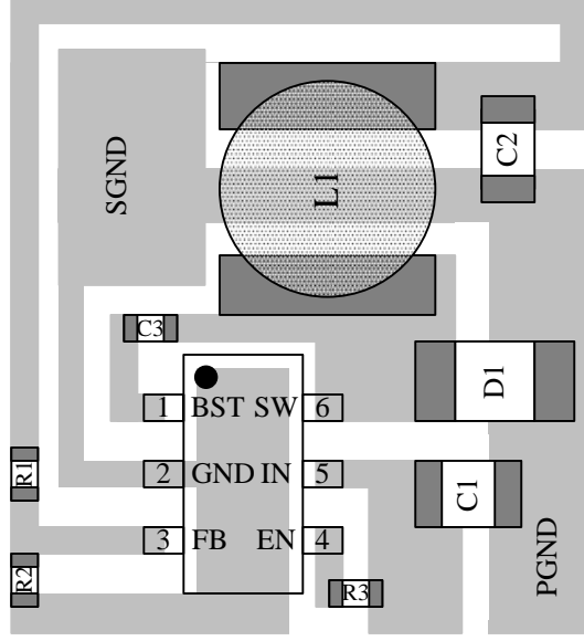
Figure 2—PCB Layout
